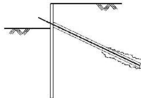
Step 3 : Drill borehole, place anchor and grout
